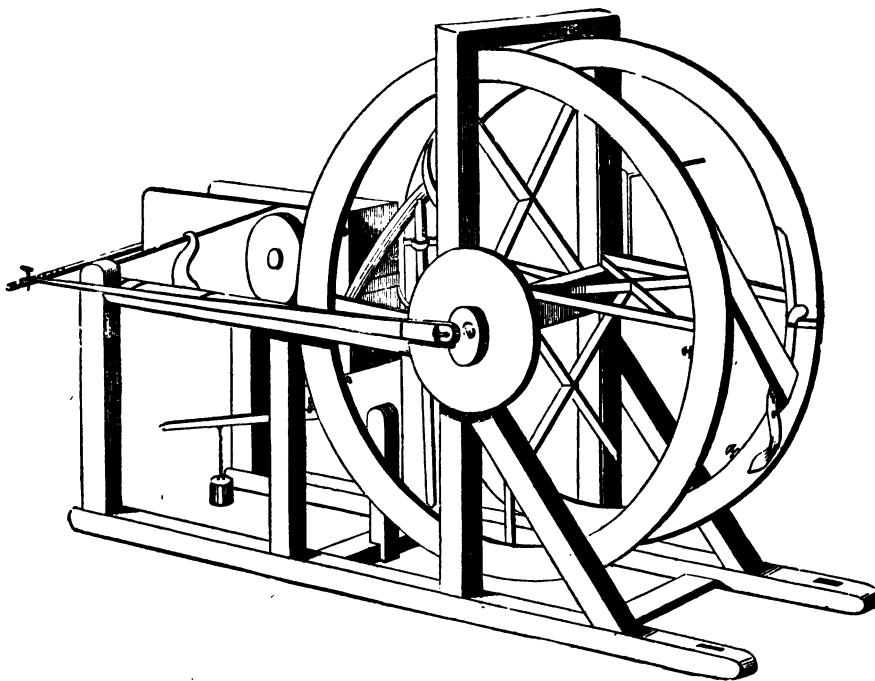
SALMON'S STRAW-CUTTER.
